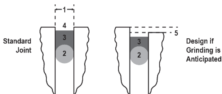
Figure 2: Recommended Joint Designs.
