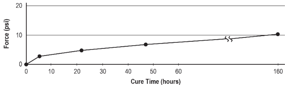
Figure 1: Cure Rate of DOWSIL™ 902 RCS Joint Sealant. 1
